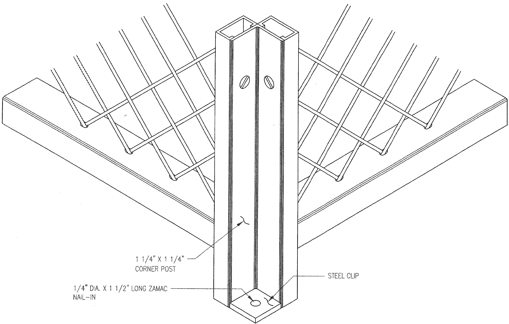
② CORNER POST NOT TO SCALE
