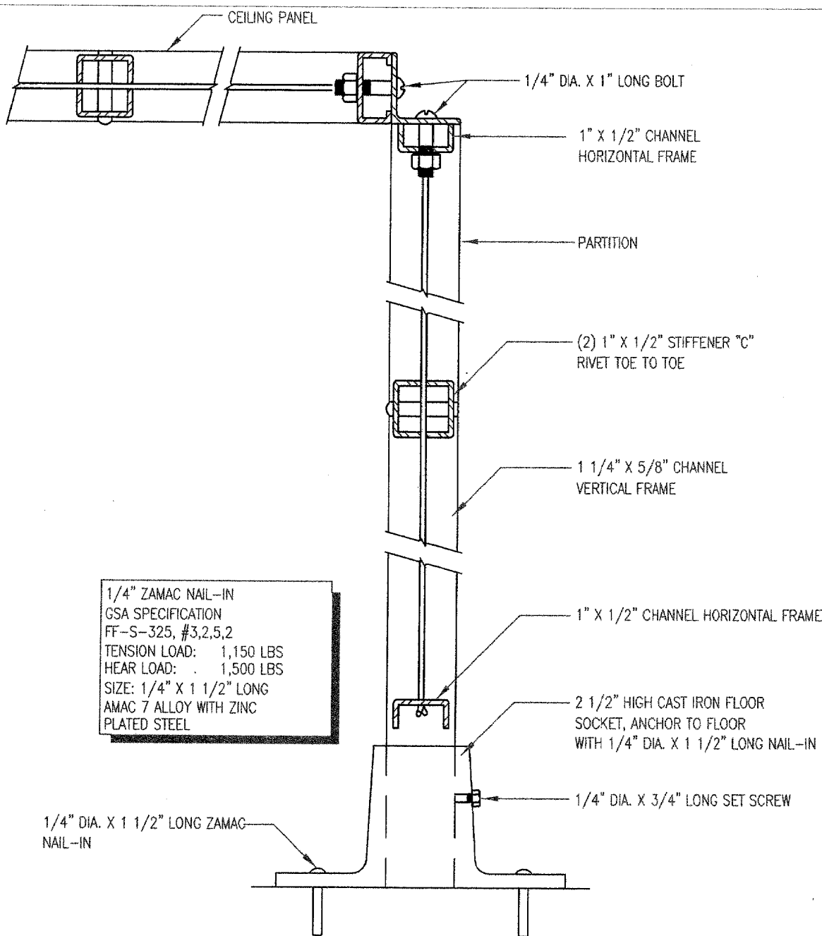
① TYPICAL PARTITION WITH CEILING NOT TO SCALE
